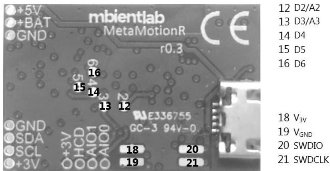
Figure 3 Back Pin Assignments
