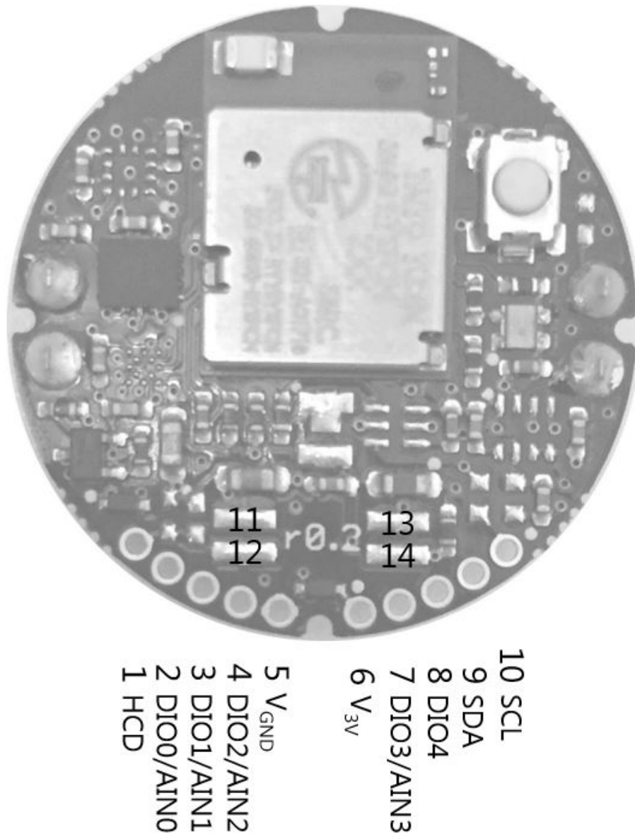
Figure 2 Pin Assignments
